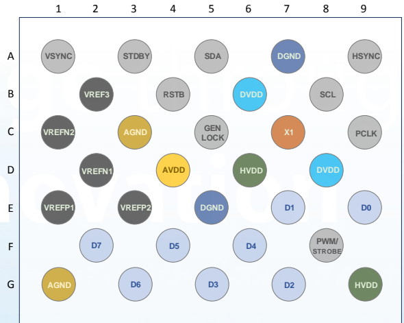
Package Top View For DVP
