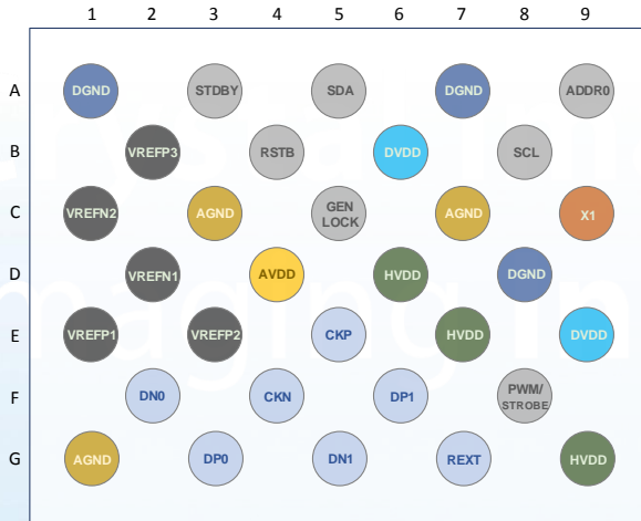
Package Top View For MIPI
